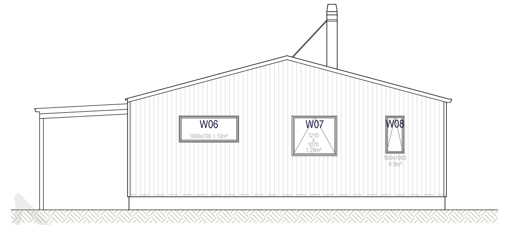
WEST ELEVATION
