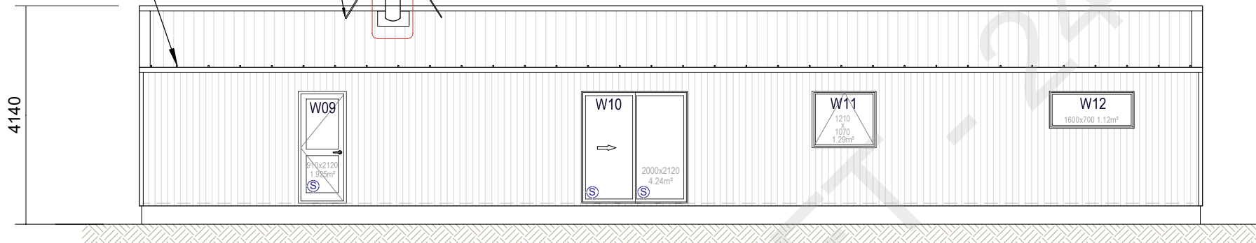
SOUTH ELEVATION
